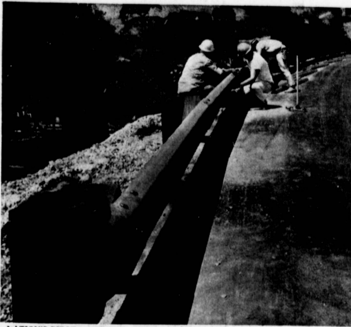
NATION'S FIRST... Steel channels produced at U. S. Steel's Torrance Works are part of a 655-ton contract for the first large scale installation of Cor-Ten freeway median barriers and guard rails. Some 20 miles of the high-strength weathering steel which needs no painting will be installed on the Junipero Serra Freeway in San Francisco.
