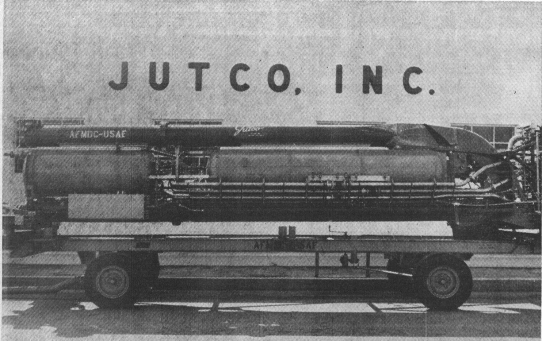
MISSILE SLED has been delivered to the Air Force Missile Development Center, Holloman Air Force Base, by Jutco, Inc., 122 E. 162nd St., Gardena. The sled will push missile and satellite components down a seven-mile track to simulate forces encountered during missile launch or impact.
