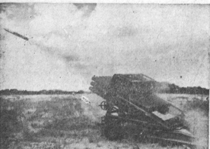
CHEMICAL AGENT ROCKET departs from Army M55 Weapons System launcher. Recently developed by the Chemical Corps, Ordnance Corps and Arthur D. Little, Inc., the lightweight aluminum weapon can be assembled, loaded and fired in less than 20 minutes.
