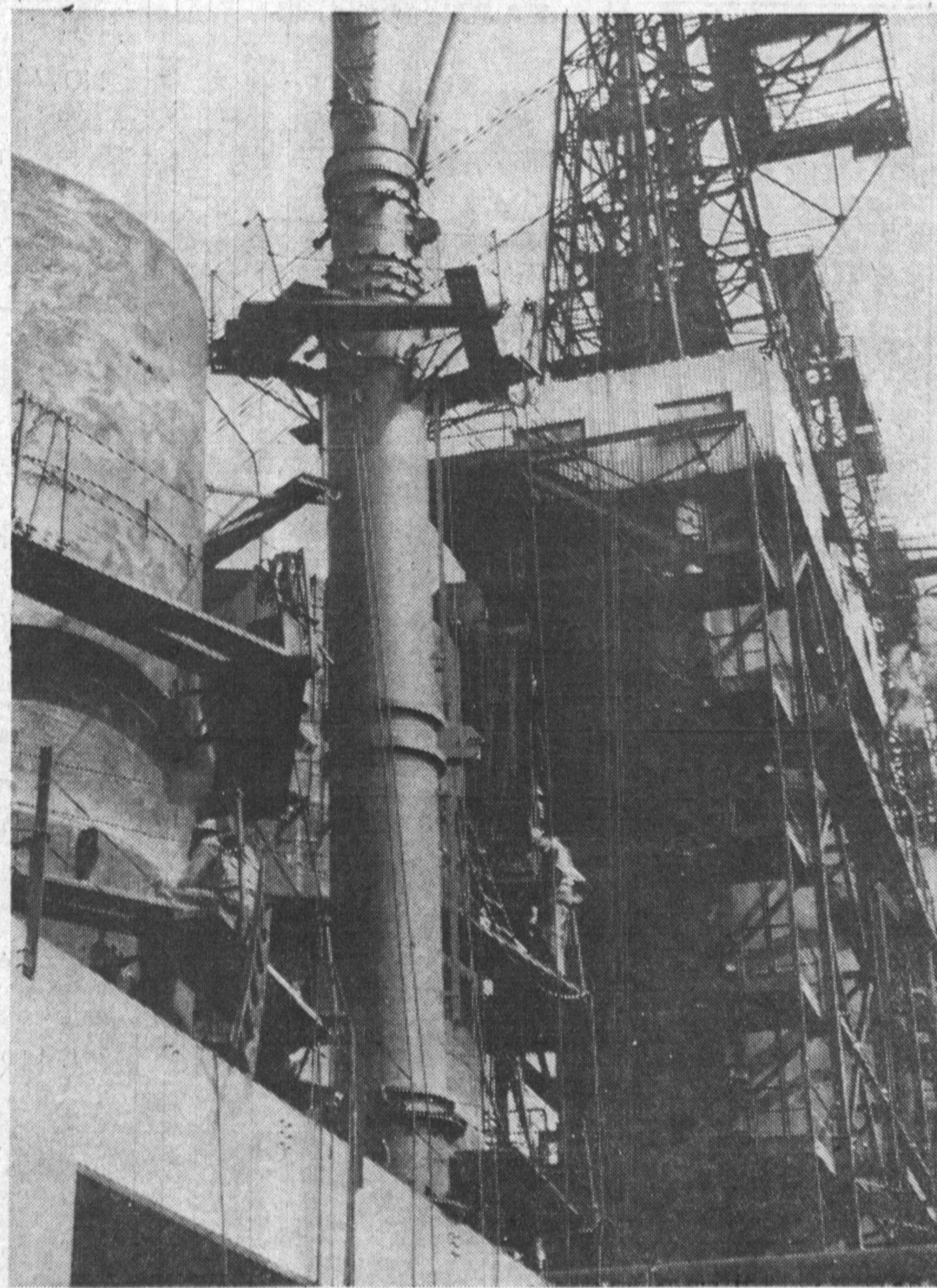
GP COKER EXPANSION UNDER WAY —In this photograph, taken from the ground, construction men are working on two drums which are part of the new coking facilities at General Petroleum Corporation's Mobil refinery at Torrance. When completed, the new unit will have a planned throughput of 9300 barrels a day, increasing refinery's coking capacity to 35,000 barrels a day.
