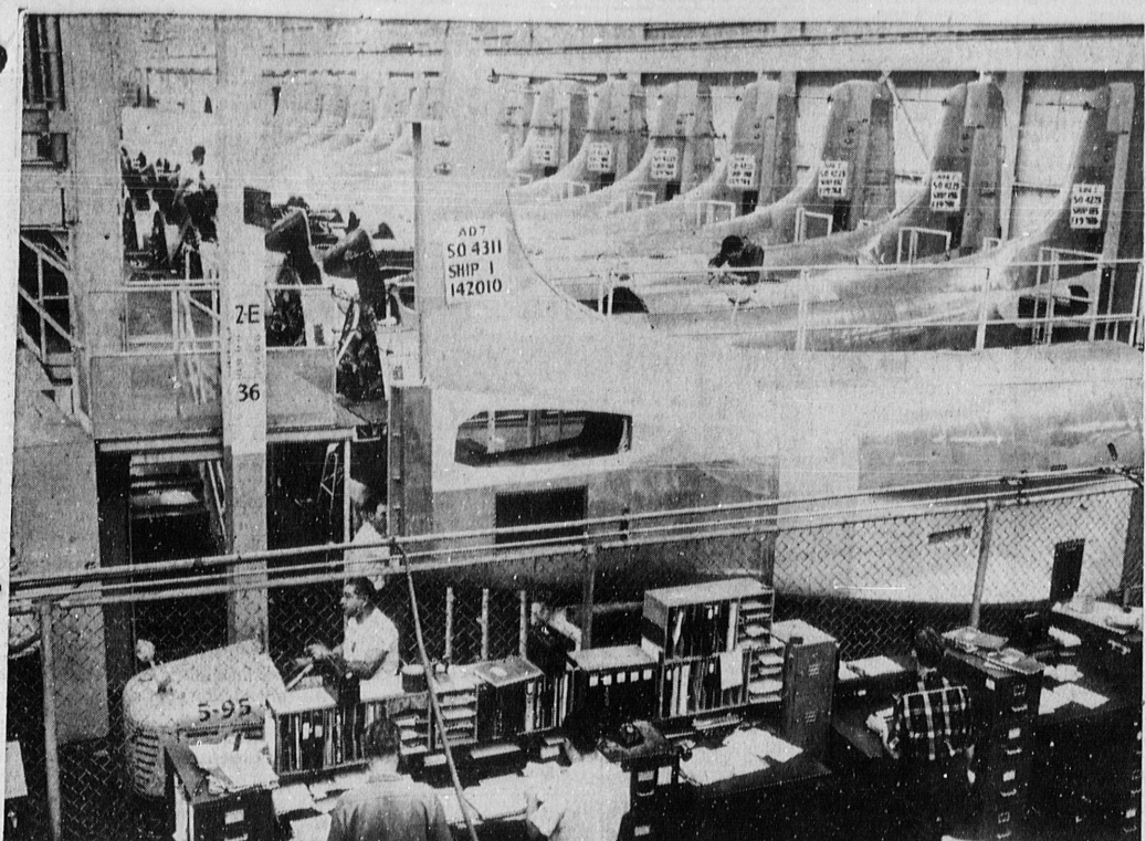
SHIP ONE... First AD-7 fuselage to be delivered to Torrance joins a line of its predecessor, the AD-6. All electric, hydraulic, and control systems will be installed and the fuselage joined to the center wing. Final assembly will be completed at El Segundo.
