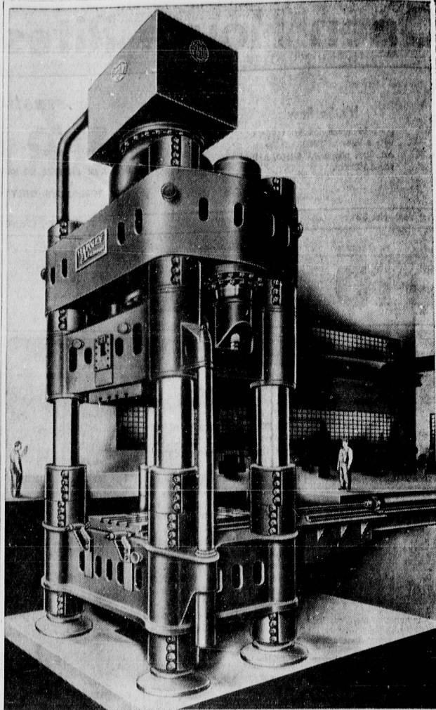
INDUSTRIAL GOLIATH ... This 8000-ton hydraulic forging press, one in a complement of new presses being installed at the Harvey Aluminum plant here incorporates the most advanced innovations in forging equipment. A part of the Air Force Heavy Press Program, the machine is extremely rigid in design, will restrict full load deflection to a minimum, and will accommodate complex unsymmetrical forgings. Designed for the most advanced production requirements of the airframe industry, the press will permit Harvey to produce precision, no-draft forgings accenting thin webs and ribs, close tolerance, etc.
