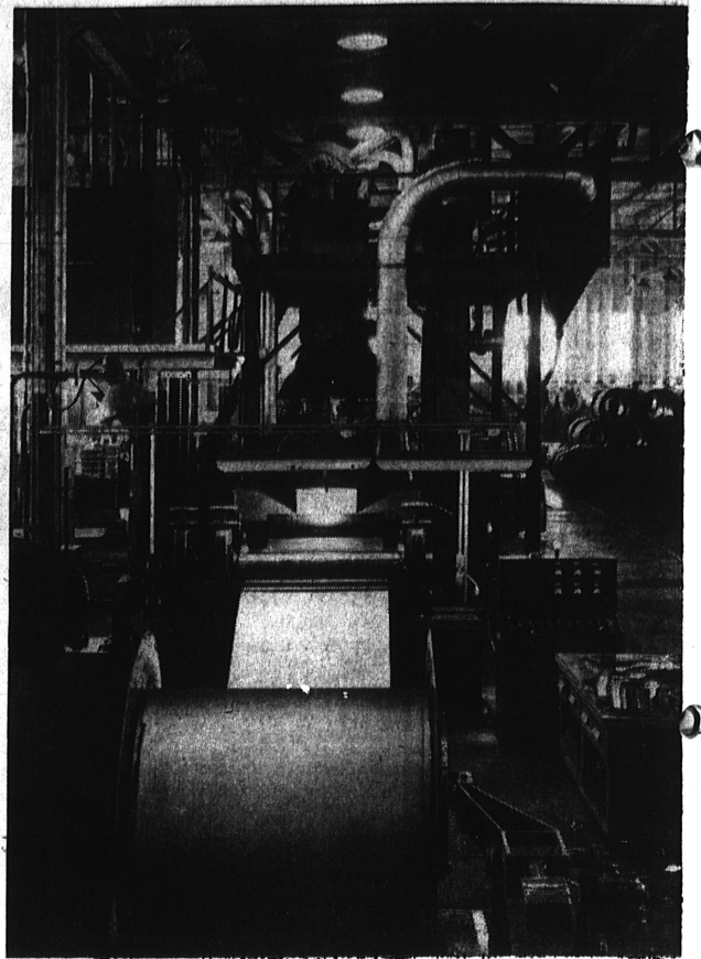
FRONT OF THE LINE . . . This is the first step in the manufacture of Rome Cables' rigid Conduit. Here is the sheet steel going through the rigid conduit shot blast cleaning and sitting line.
