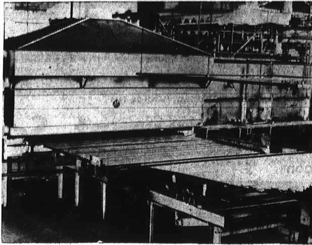
A ROME HOT DIP . . . After forming, the conduit goes into the Sendzimir hot dip galvanizing and annealing process. Here the already formed conduit is being fed by automatic tables into the Sendzimir furnace.
