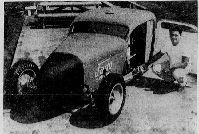
BUILT FOR SPEED . . . Jim Kamboor poses by the side of "Jado," the racing car with which he won third place in the Class B division of the Bonville Speed Races recently. Never road tested before it was run, the car went 164 miles an hour.
