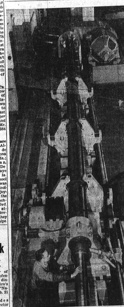
MAN SIZED JOB... Trepanning a 3 1/2-inch diameter bore in a 41-foot shaft on the 124-foot long trepanning lathe at the local National Supply Co. plant is speeded up with the speed increasing device driven by 25 V-belts off the 150 horsepower motor. In trepanning, a hole is produced by removing a core, much the same manner as an apple is cored. The speed increasing device is at the upper right hand corner of the picture along with the huge electric motor which powers the lathe.
