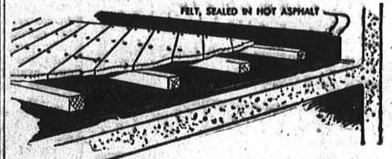
With concrete slab construction, an underfill of cedar or washed gravel is usually necessary. Also use a felt waterproofing membrane.
