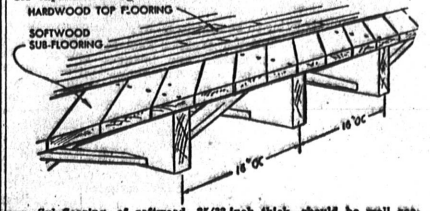
Sub-flooring of softwood, 25/32-inch thick—should be well seasoned, laid diagonally with two 16d nails at each joint and board end.
