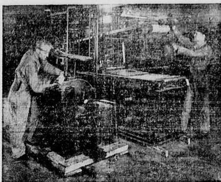
CONSTRUCTION CREW... assembles automatic Ford tire builder which will take its place on the production line at the Los Angeles plant of the United States Rubber Company.
