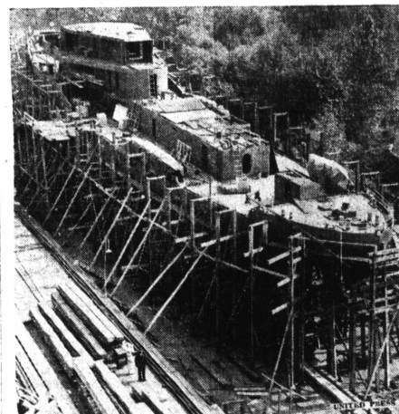
SURVEY SHIP NEAR COMPLETION . . . Little discussed but actually a major key in the new National Defense program is this new U. S. Coast and Geodetic Survey ship, the "Explorer," rapidly nearing completion at the shipyard on the east side of Lake Washington, near Kirkland, Wash. The $1,250,000 vessel will be 220 feet long, 38 feet wide, and will develop 14 knots with her 2,000 horsepower engines. The "Explorer" will be used as a survey ship around the Alaska coast and the Hawaiian Islands, mapping out National Defense locations. Twenty-three officers and 70 men will comprise the crew.
