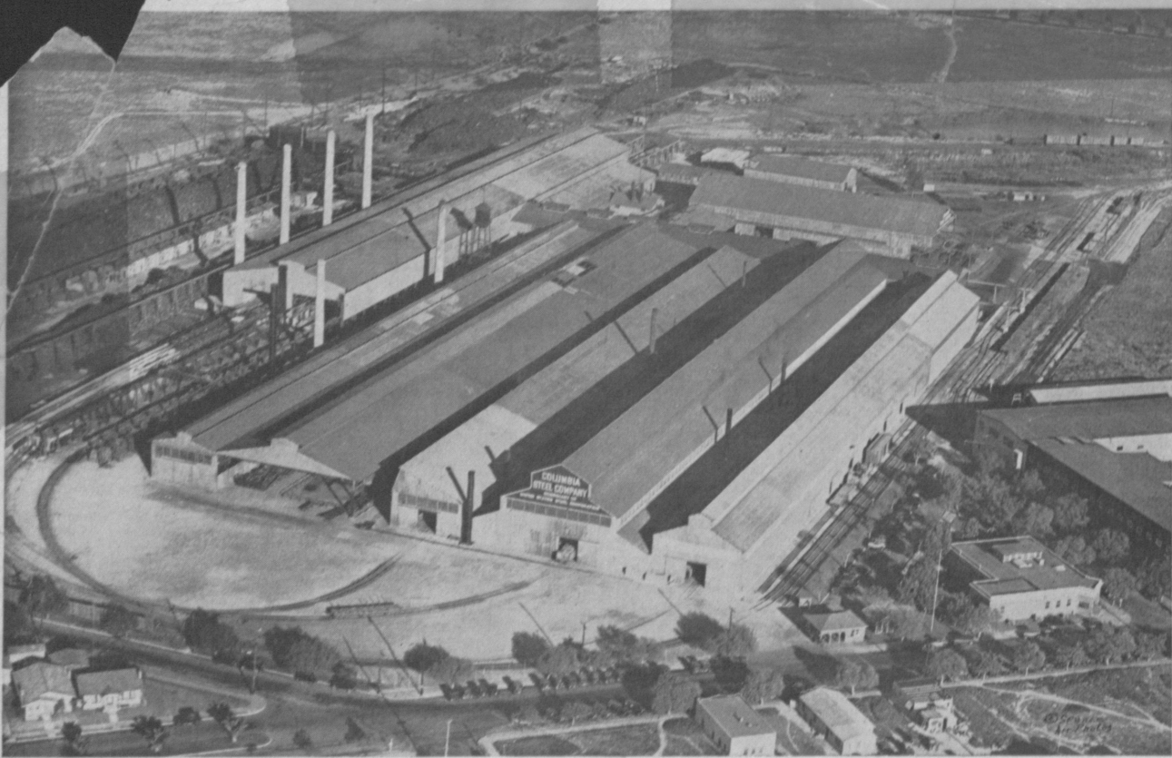
Airplane view of Torrance, California, Plant of Columbia Steel Company
