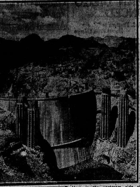
Here is the upstream side of Boulder Dam as seen from a high point on the Arizona rim of Black Canyon. The intake tower on the right on the Nevada side, is already completed, while the other three are nearing completion.
