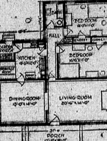
THE KEOTA—DESIGN A523
